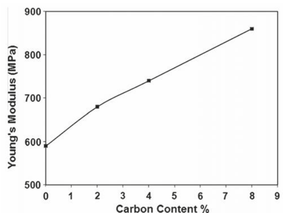
Figure 1: Influence of carbon nano-particles percentage on Young's modulus of HDPE matrix (from Characterization and processing of high density polyethylene/carbon nano-composites. H. Fouad, Rabeh Elleithy, S. M. Al-Zahrani, Mohammad Al-haj Ali. Materials and Design, Vol. 32 , 2011, pp1974-1980).
